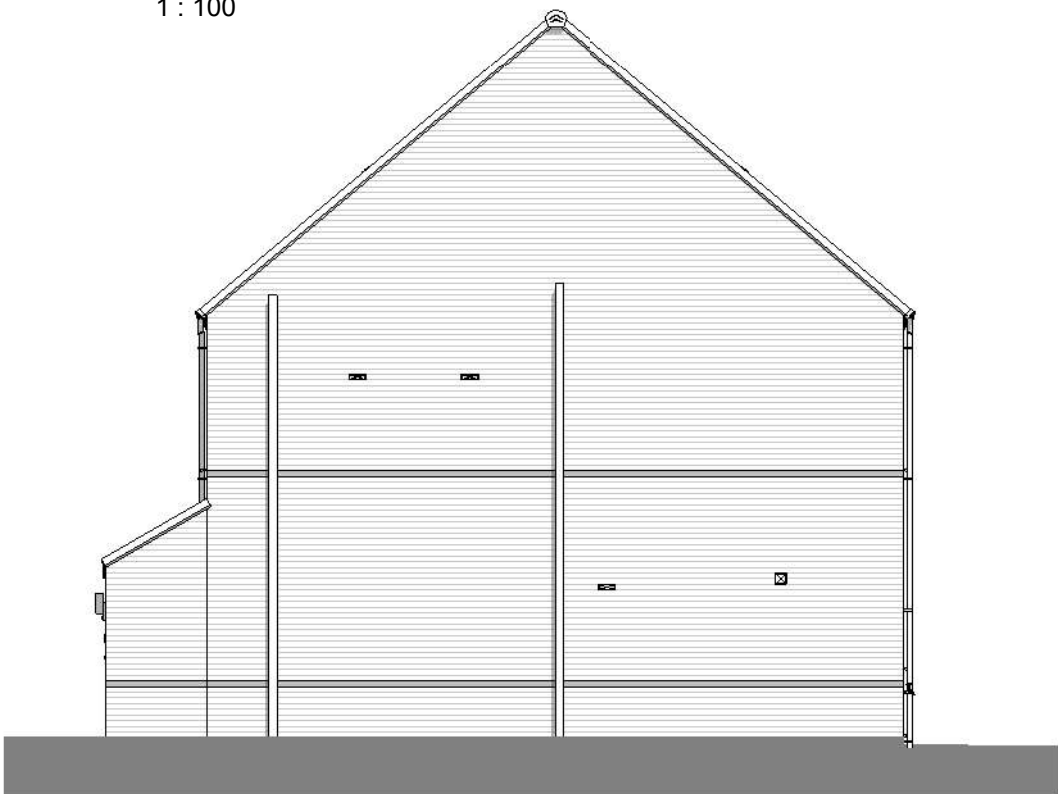
Rear Elevation 1 : 100
