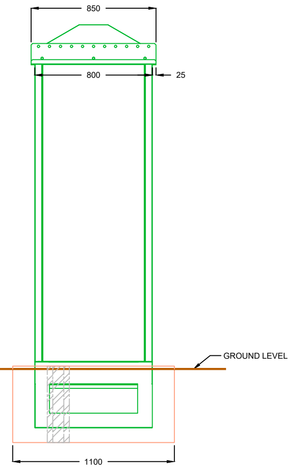
SIDE ELEVATION (LEFT - DOORS CLOSED)
