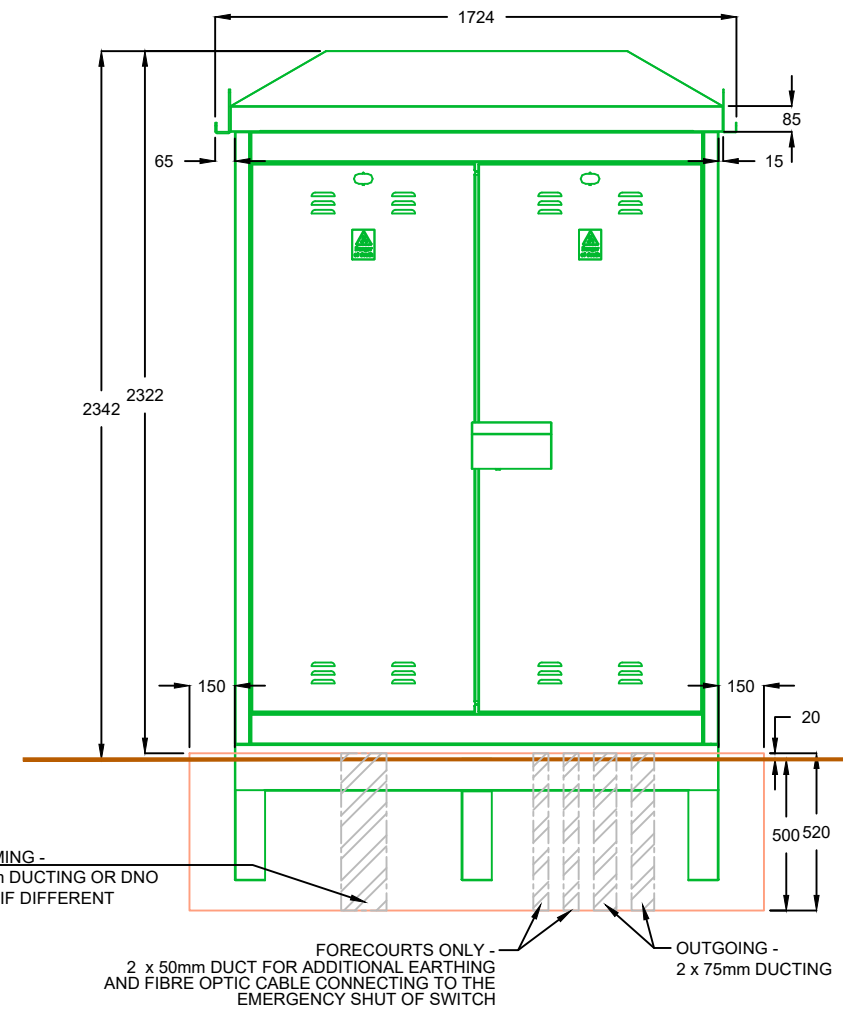
FRONT ELEVATION
