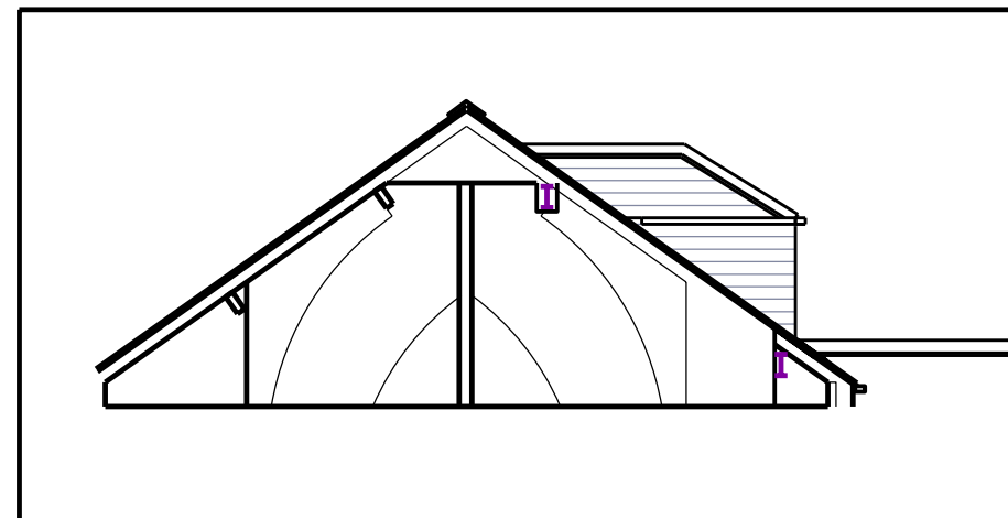
Cross Section / West Elevation - Proposed
