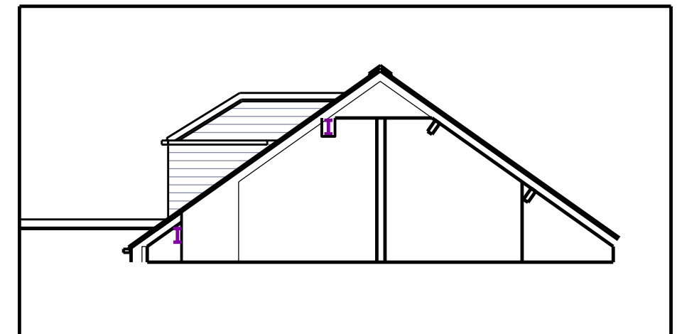
Cross Section / East Elevation - Proposed
