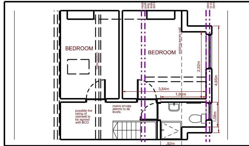
Second Floor Plan - Proposed
