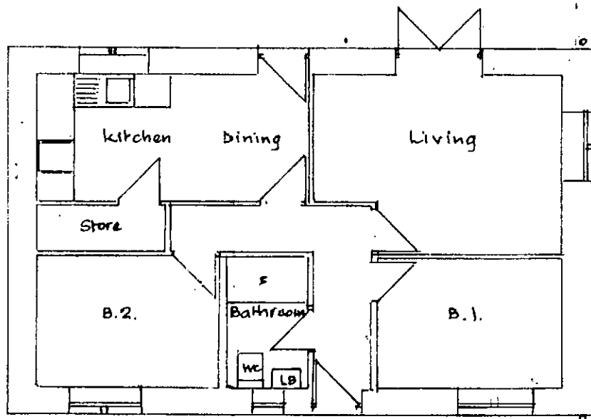
PROPOSED PLAN
