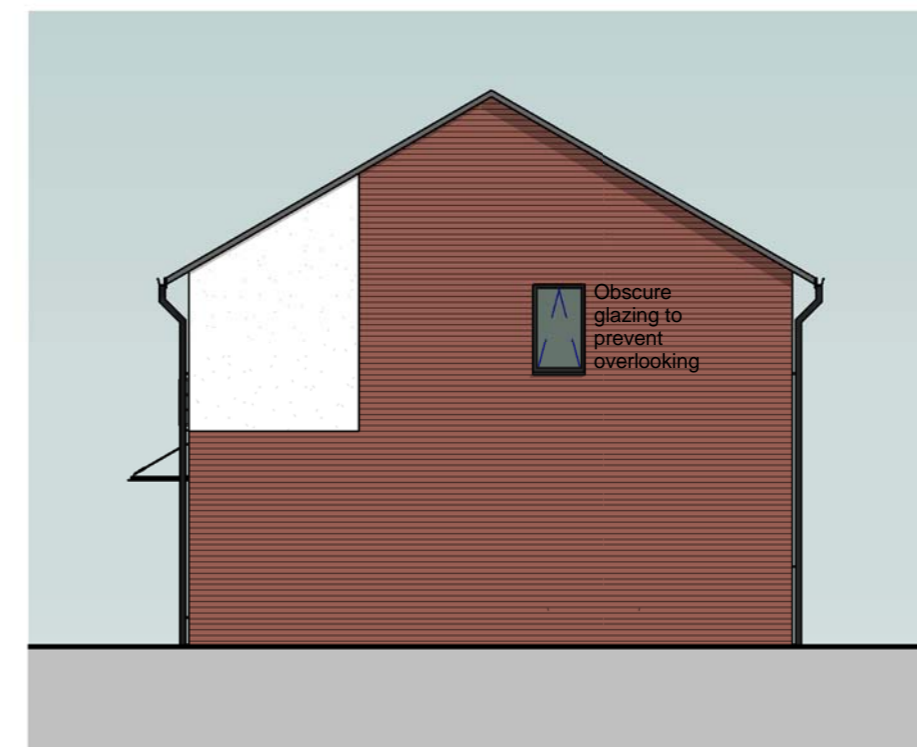
Plot 15 Side / West Elevation 1 : 100
