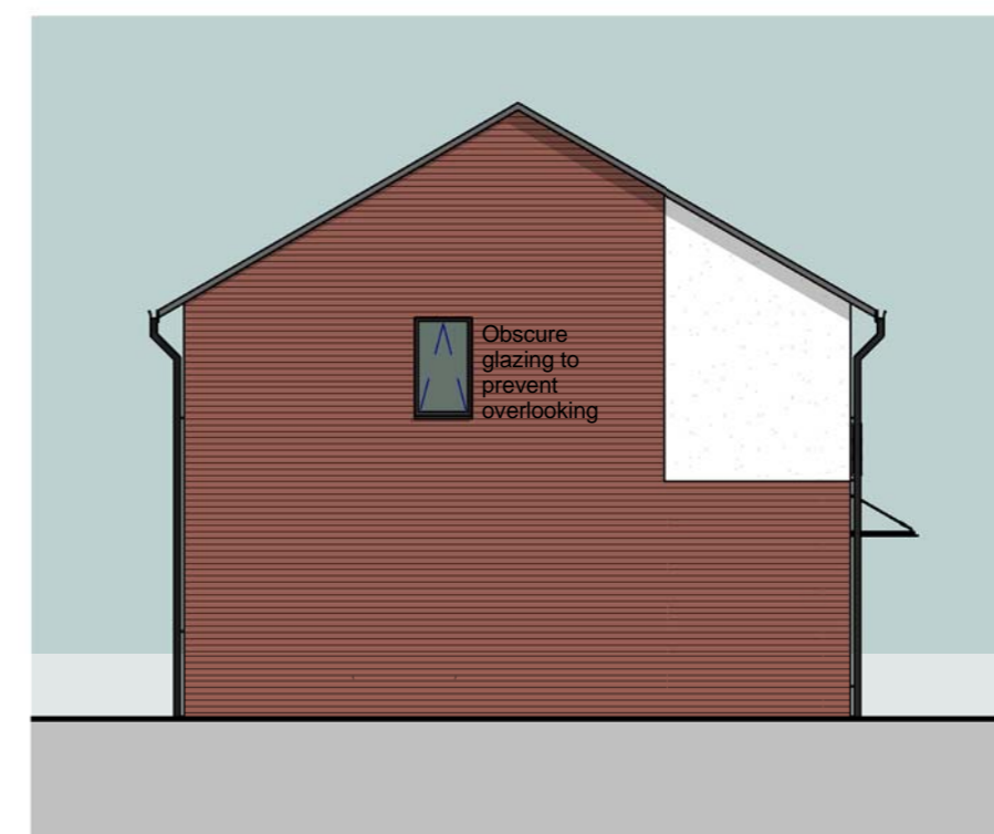
Plot 16 Side / East Elevation 1 : 100
