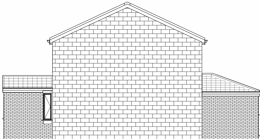
3 North Existing 1 : 100
