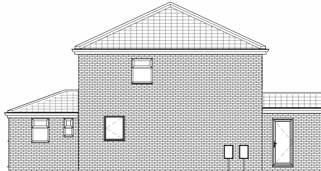
1 South Existing 1 : 100
