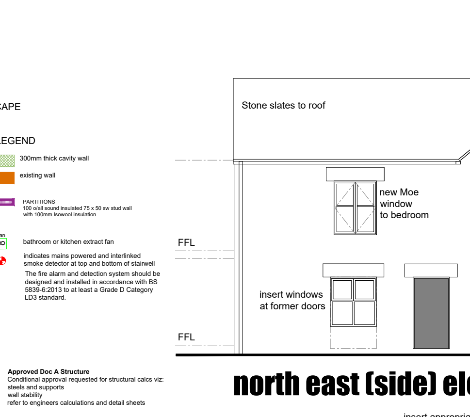
north east (side) elevation
