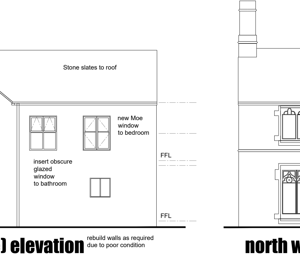
north west (side) elevation
