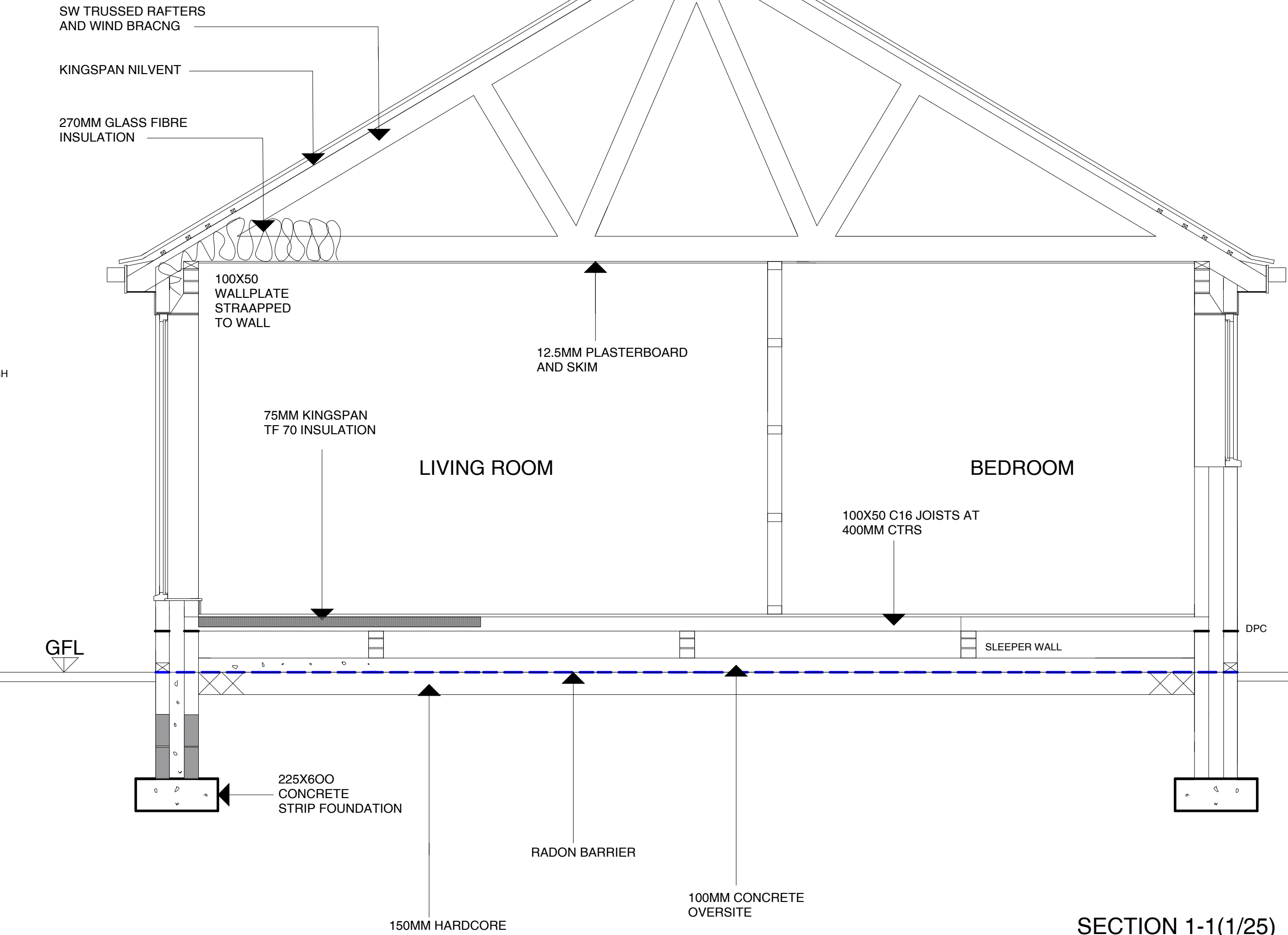
SECTION 1-1(1/25)
