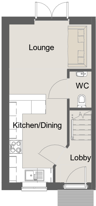
Ground Floor. 1 : 100
