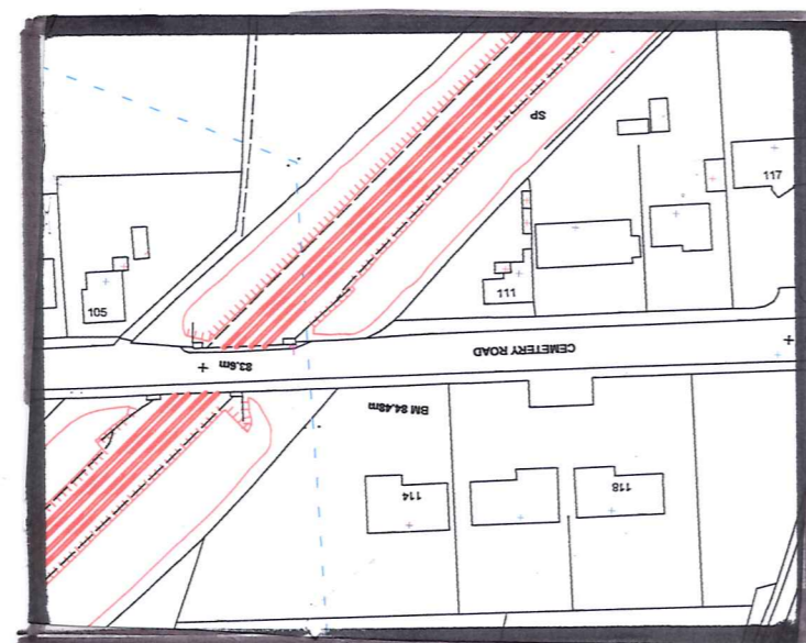
PROPOSED PLAN
