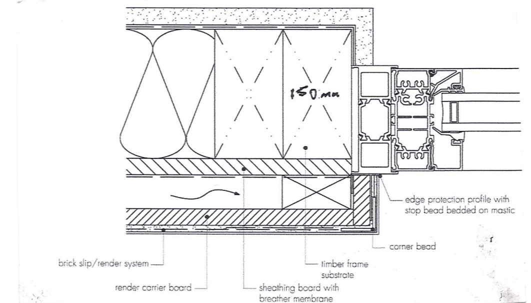
REVEAL DETAIL
