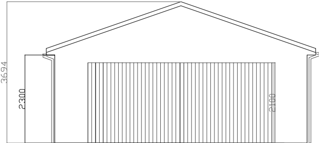
PROPOSED FRONT ELEVATION SCALE 1/100
