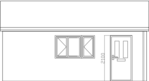
PROPOSED LH SIDE ELEVATION SCALE 1/100
