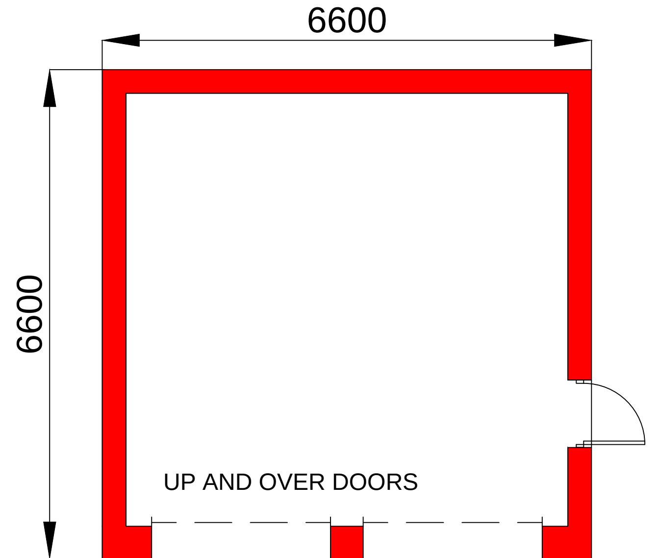
PLAN
