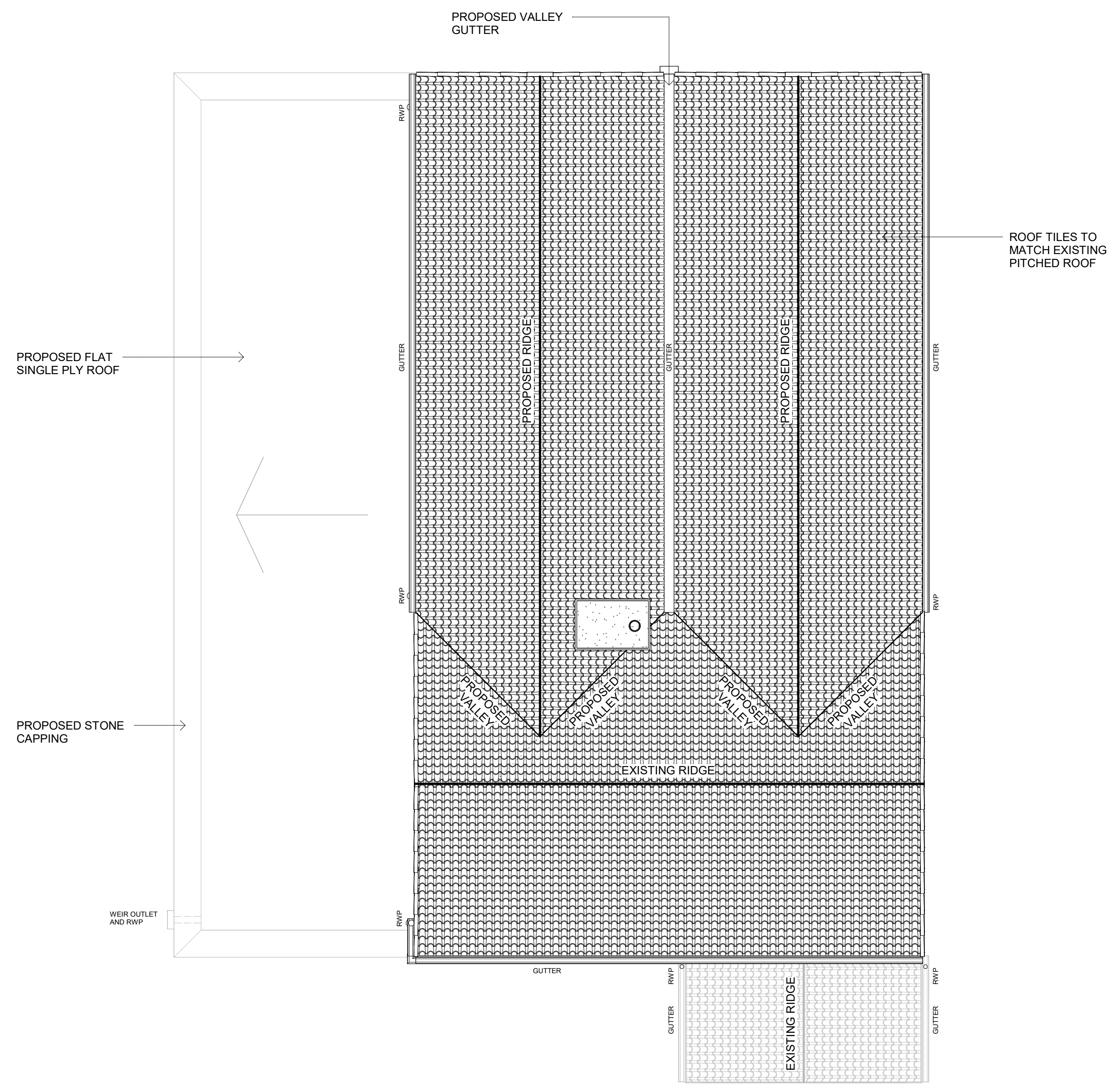
Proposed Roof Plan 1 : 50
