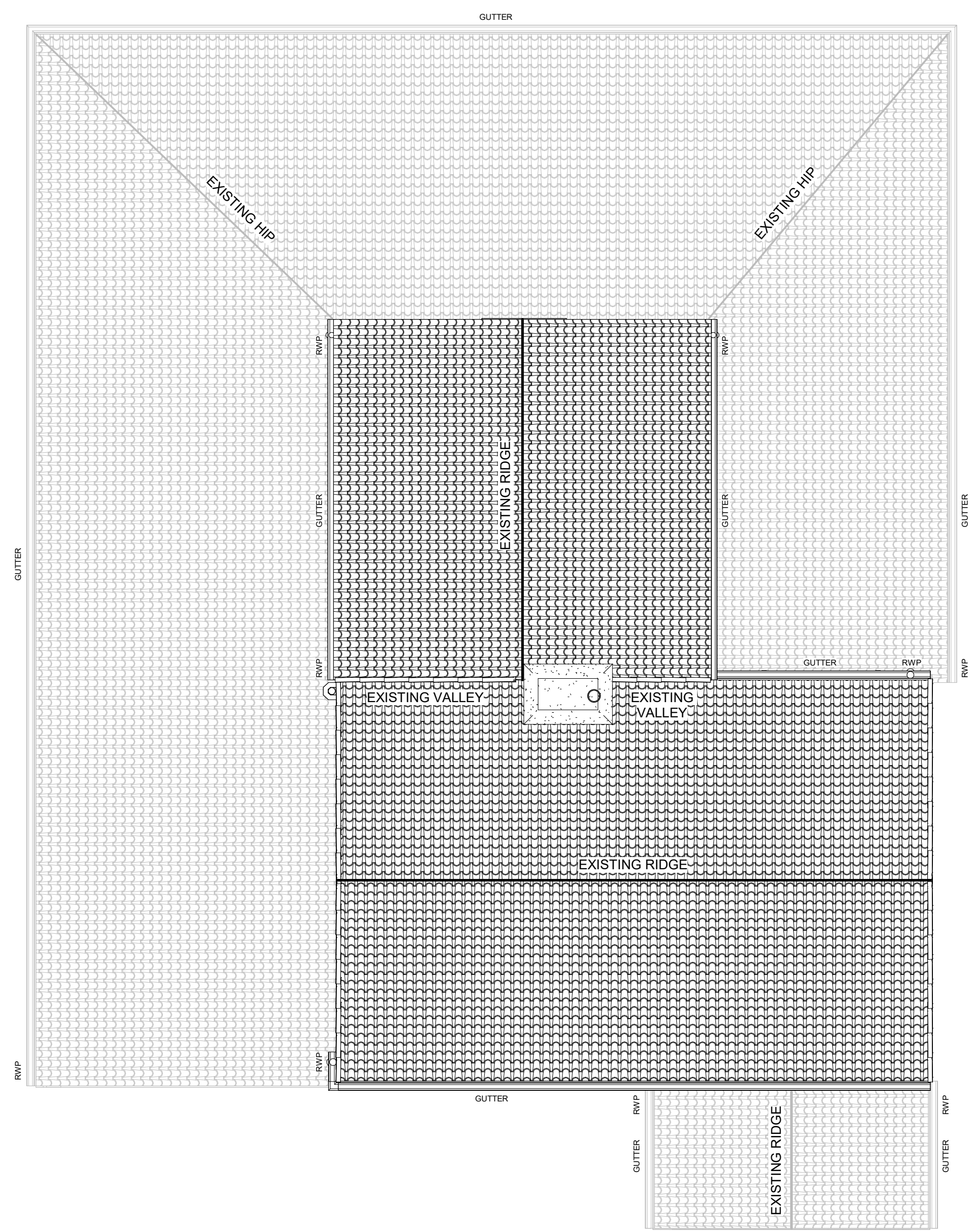
Existing Roof Plan 1 : 50
