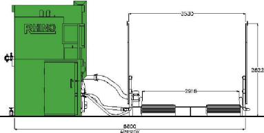
End Elevation (looking North)
