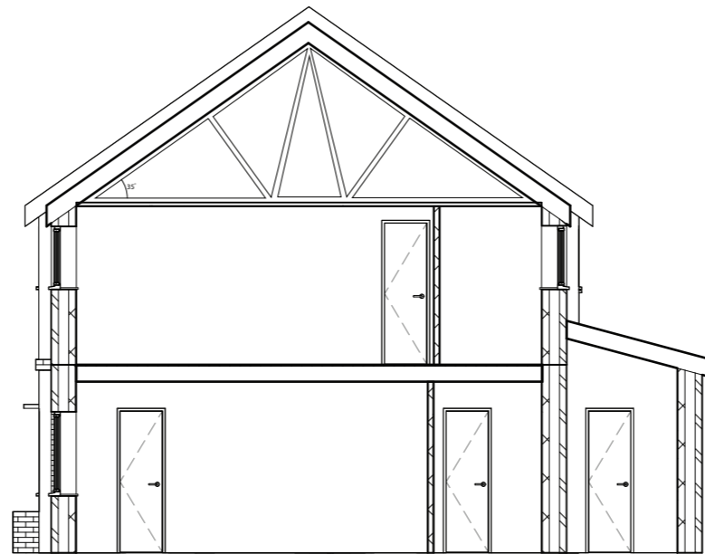
Proposed Section
