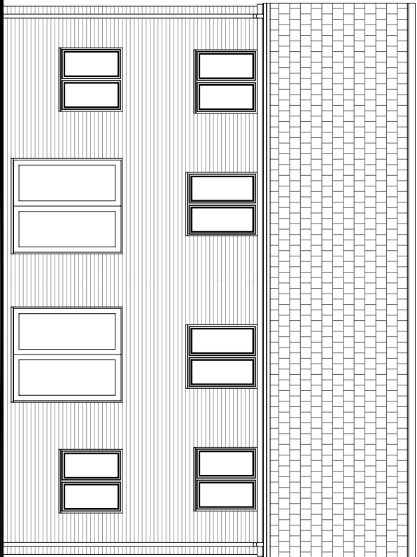
Rear Elevation
