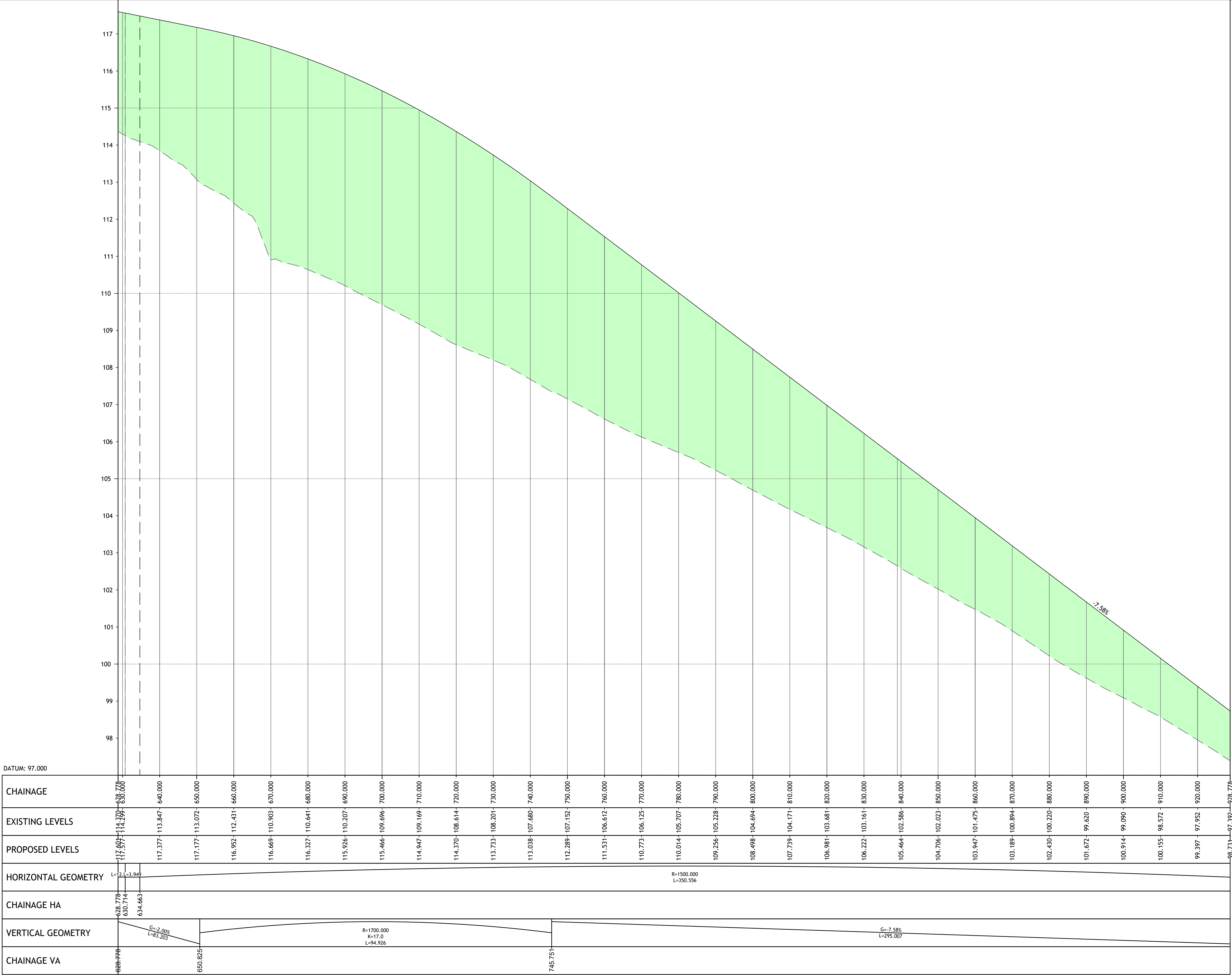
PROFILE NAME: LINK ROAD SECTION C (1 OF 2) SCALE: H 1:500,V 1:50
