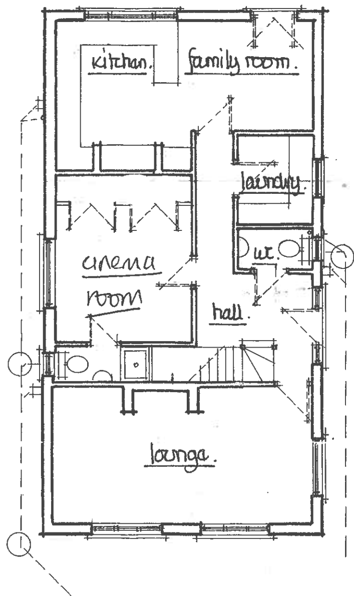
ground floor layout.
