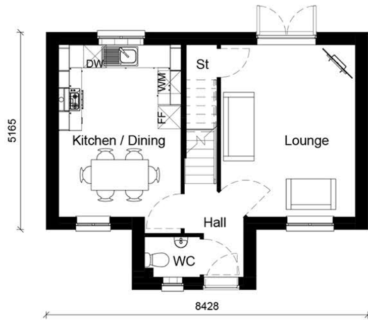
Ground Floor. 1 : 100
