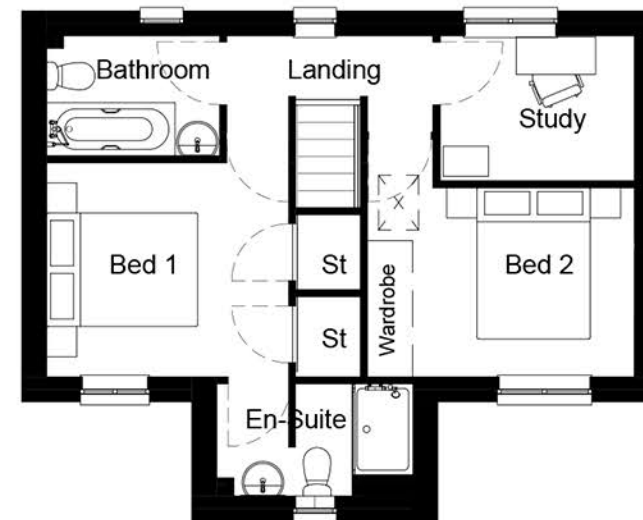
First Floor. 1 : 100
