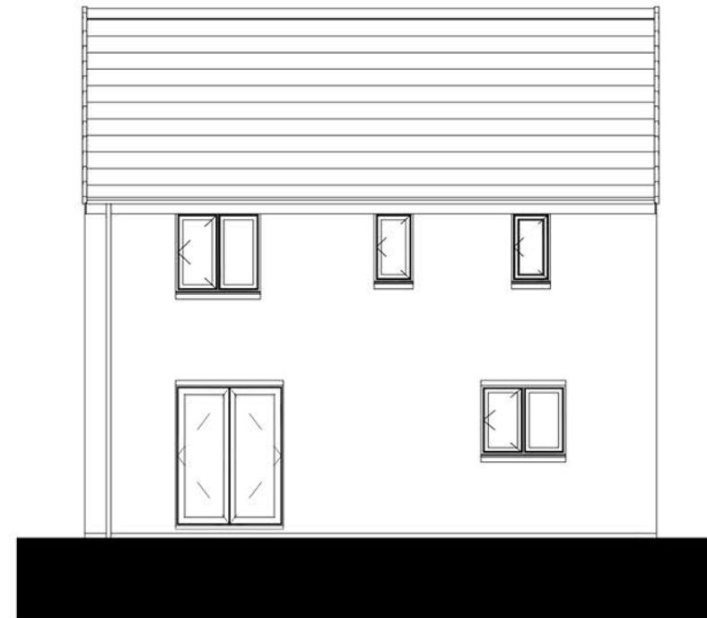
Rear Elevation. 1 : 100
