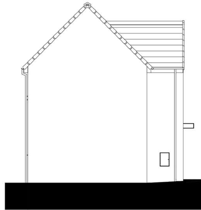
Left Elevation. 1 : 100
