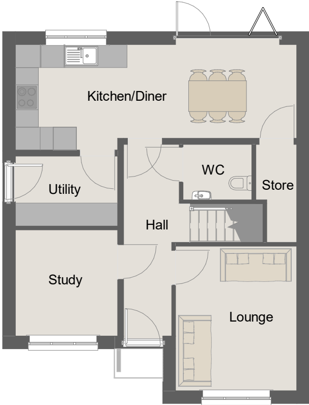
Ground Floor. 1 : 100
