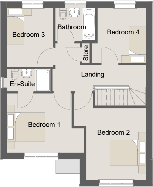
First Floor. 1 : 100
