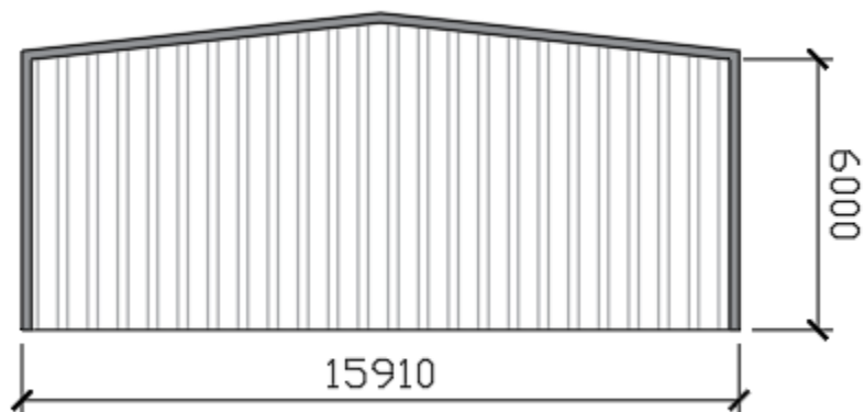
PROPOSED WEST ELEVATION
