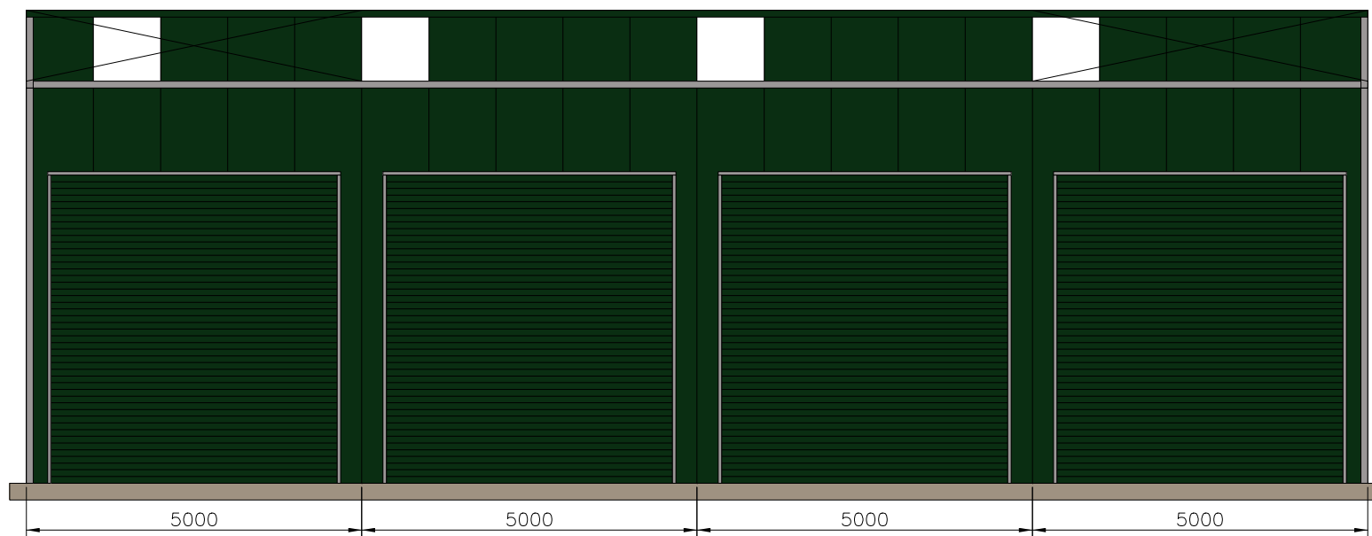
Left Elevation (Scale = 1:100)
