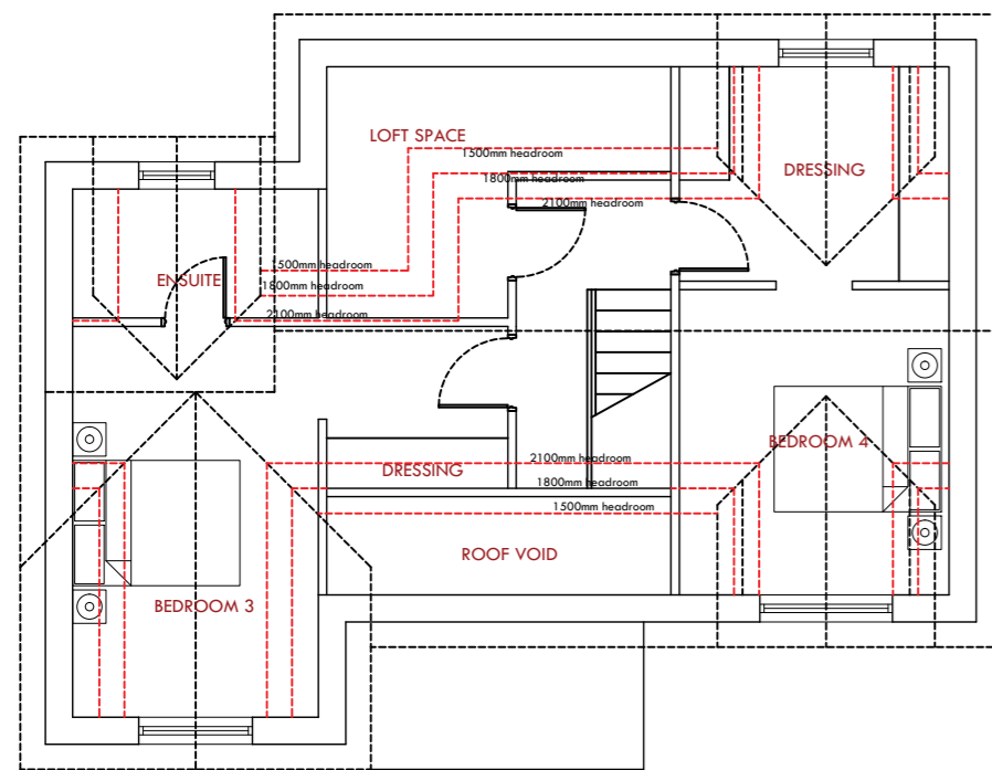
Proposed Loft Floor Plan
