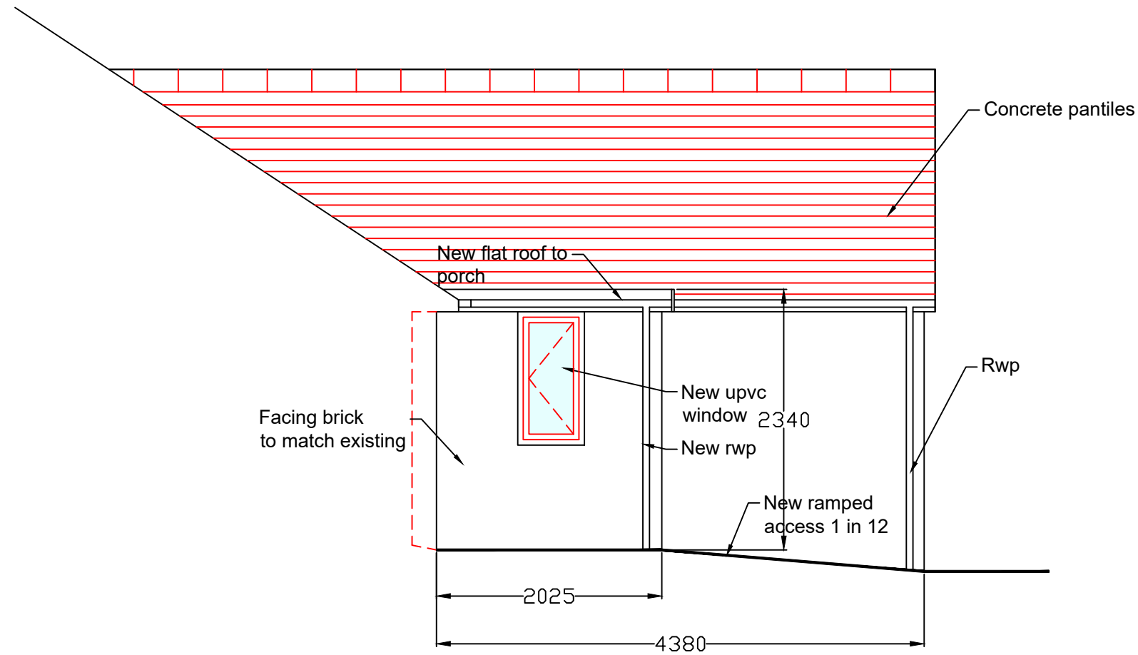
PROPOSED SIDE ELEVATION TO FRONT 1:50
