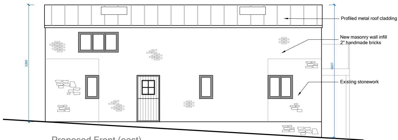
Proposed Front (east) Elevation
