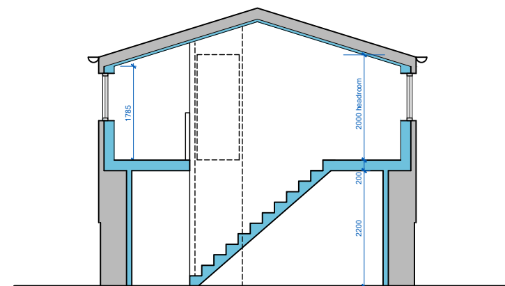
Proposed Section
