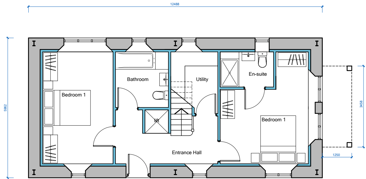
Proposed Ground Floor Plan 54 sq.m
