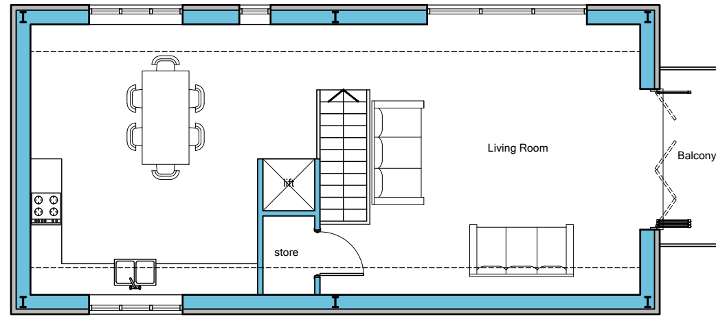
Proposed First Floor Plan 61 sq.m
