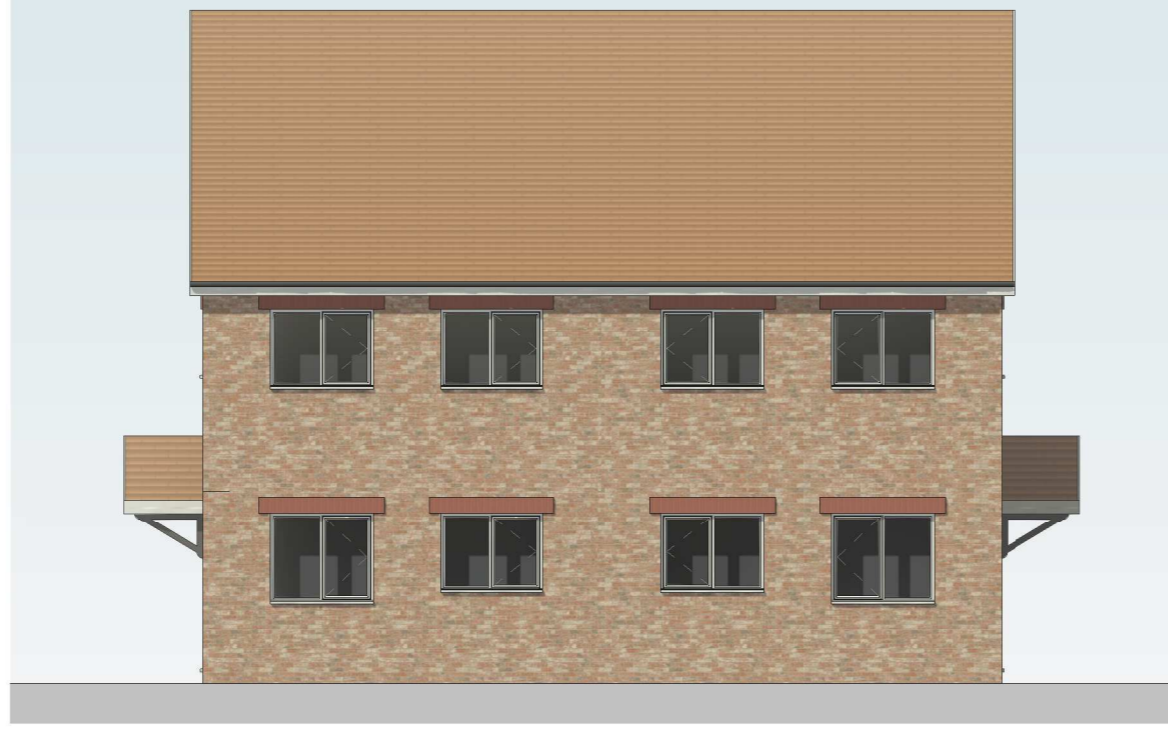
4 | APT A/B REAR_Elevation 1 : 100
