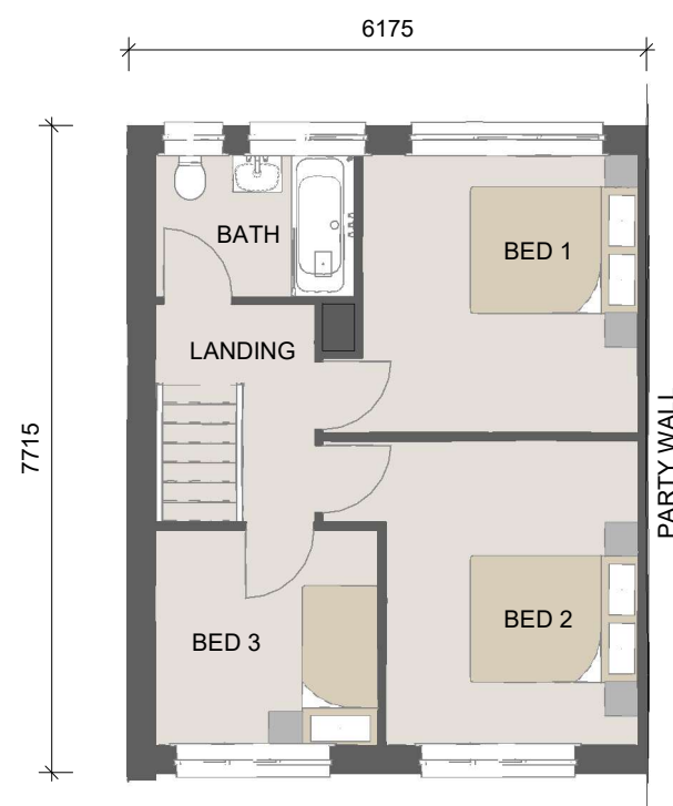
First Floor. 1 : 100
