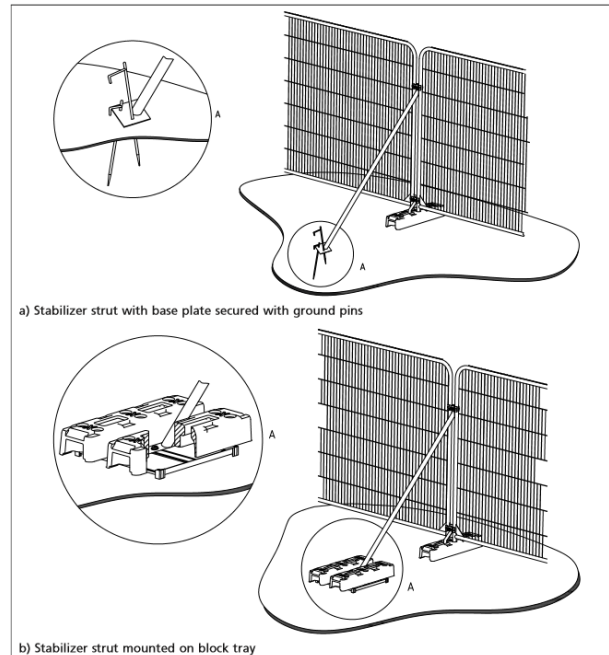
Fig 2: Examples of above ground stabilizing systems BS 5837:2012 –Trees in relation to Design, Demolition and Construction
