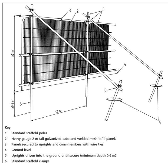
Fig 1. Protective Fencing
