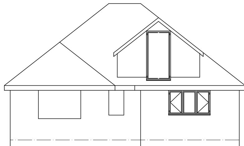
REAR ELEVATION
