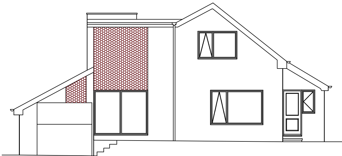
REAR ELEVATION
