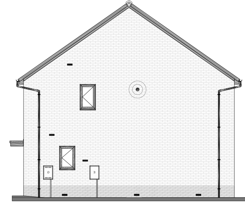
LEFT ELEVATION
