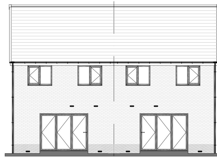
REAR ELEVATION
