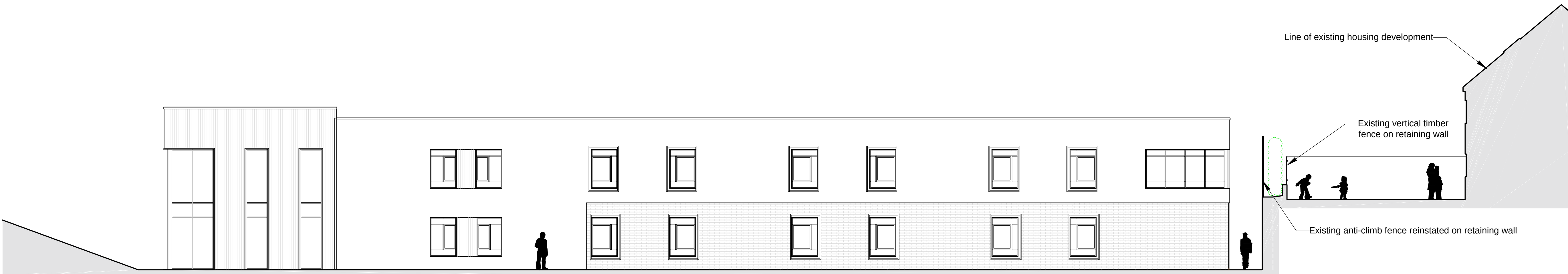
SECTION C-C SCALE - 1:100 @ A1
