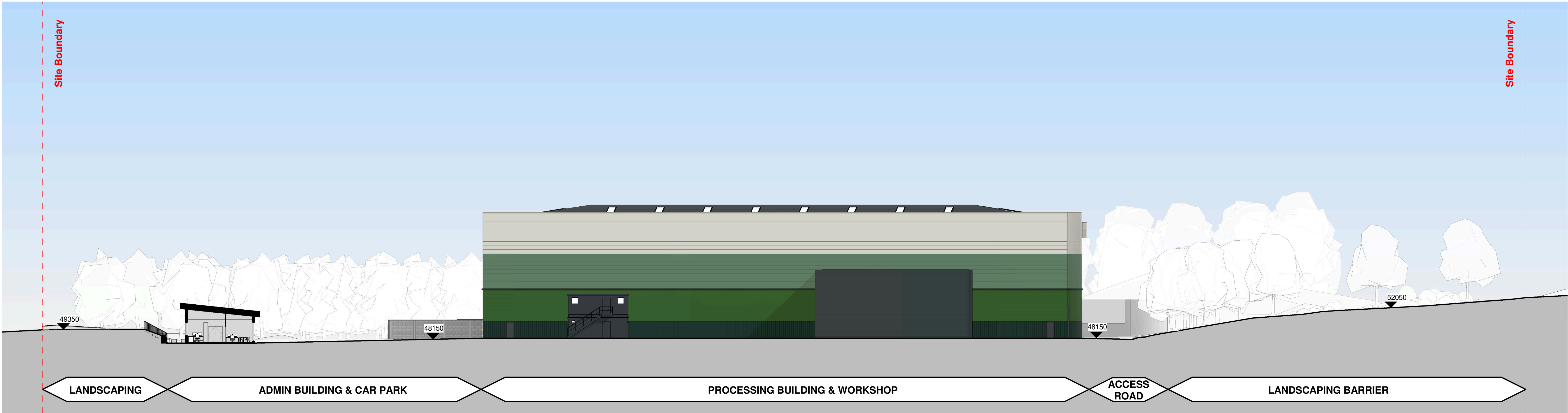
Proposed Site Section D 1 : 250
