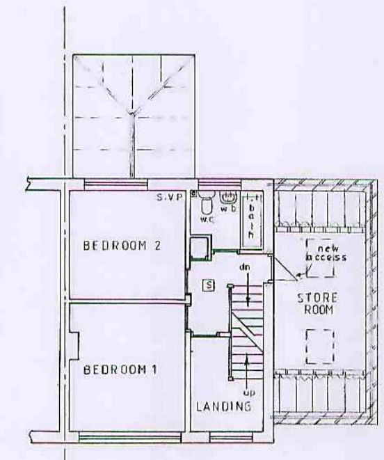
PROPOSED F.F. PLAN
