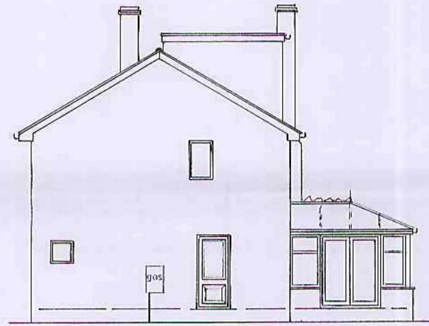
EXISTING SIDE
