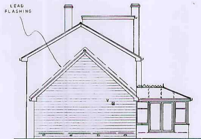
PROPOSED SIDE
