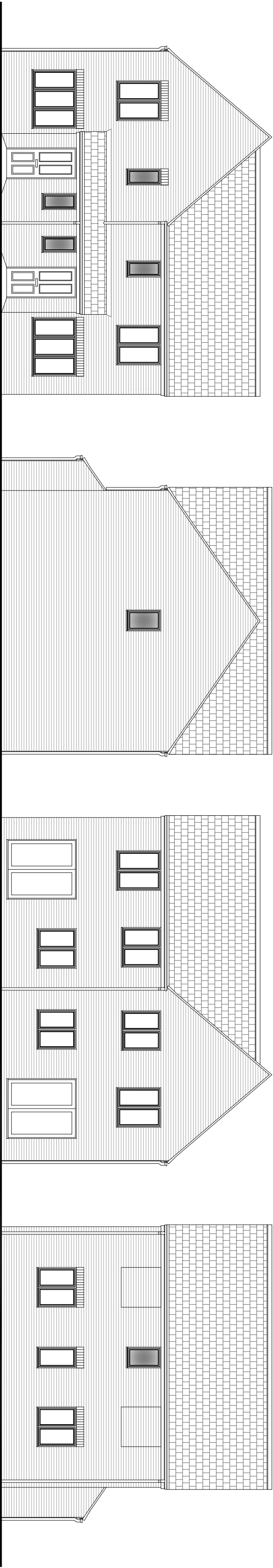
Front Elevation
