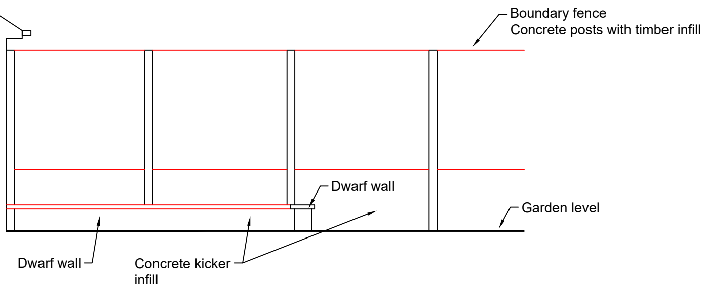
EXISTING SIDE ELEVATION TO REAR - EAST 1:50
