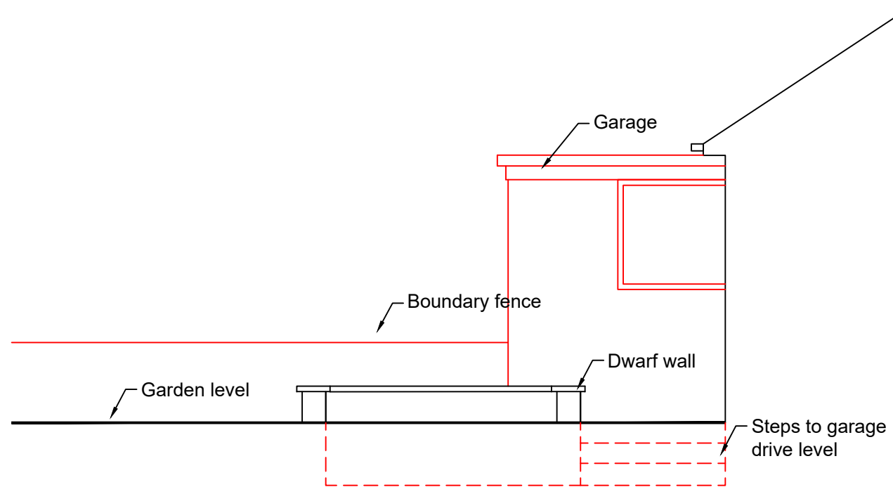
EXISTING SIDE ELEVATION TO REAR - EAST 1:50
