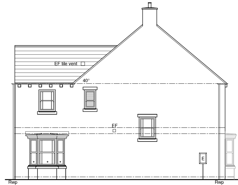
Side Elevation PS-Type-E
