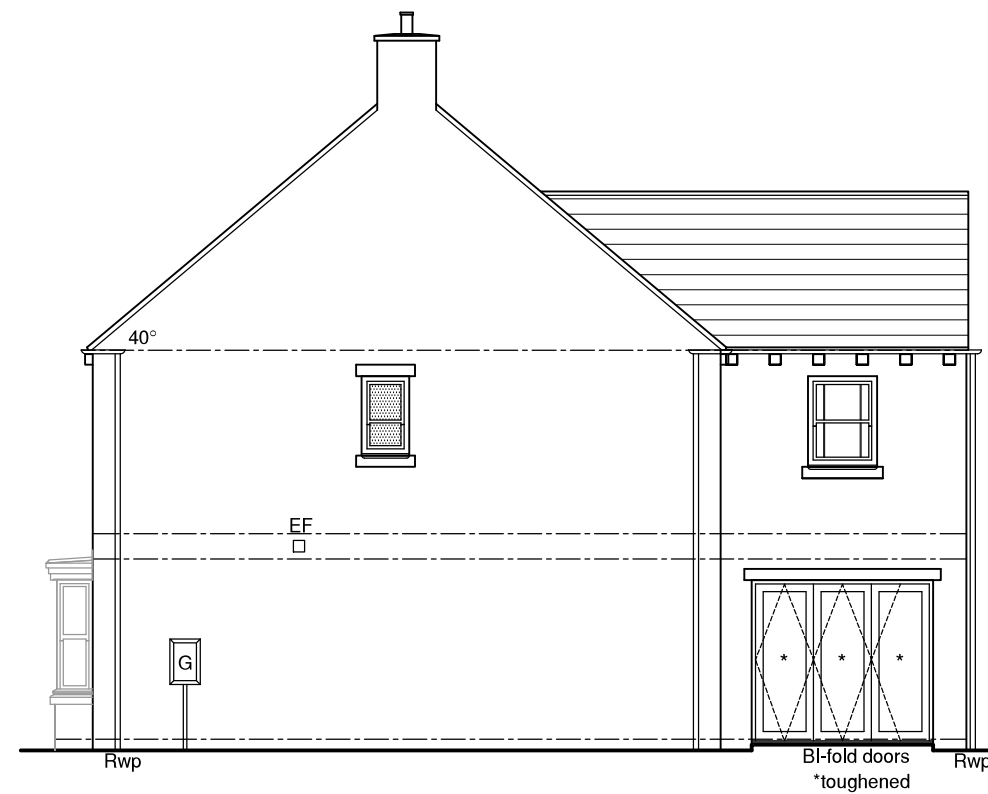
Side Elevation PS-Type-E
