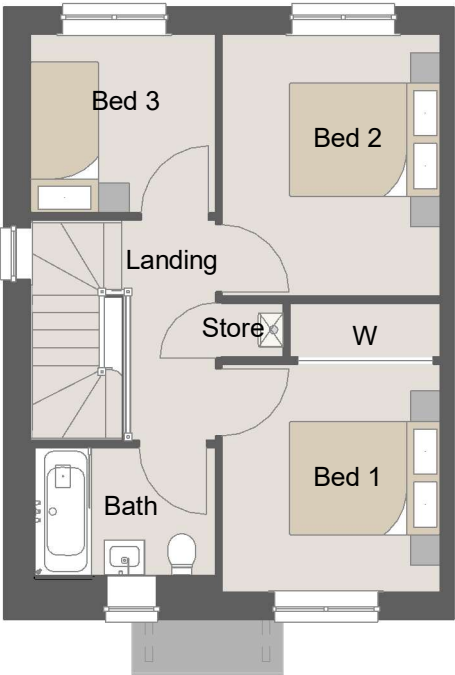
First Floor. 1 : 100
