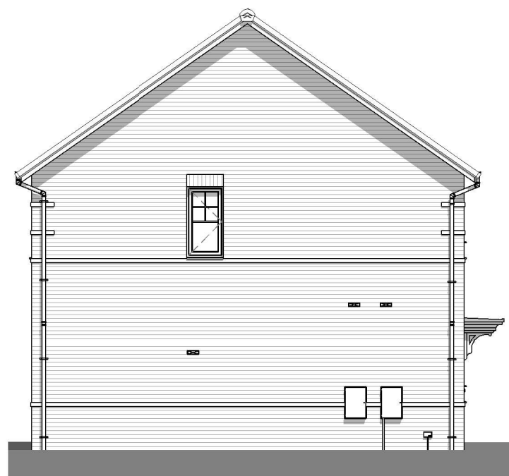
Left Side Elevation. 1 : 100
