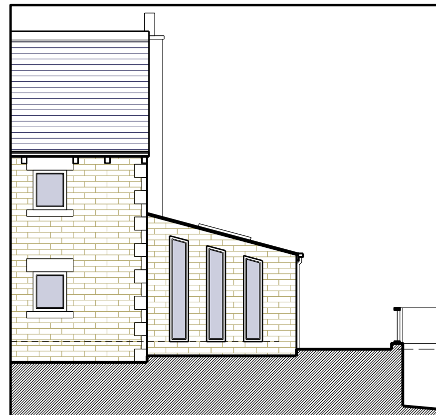
West Elevation
