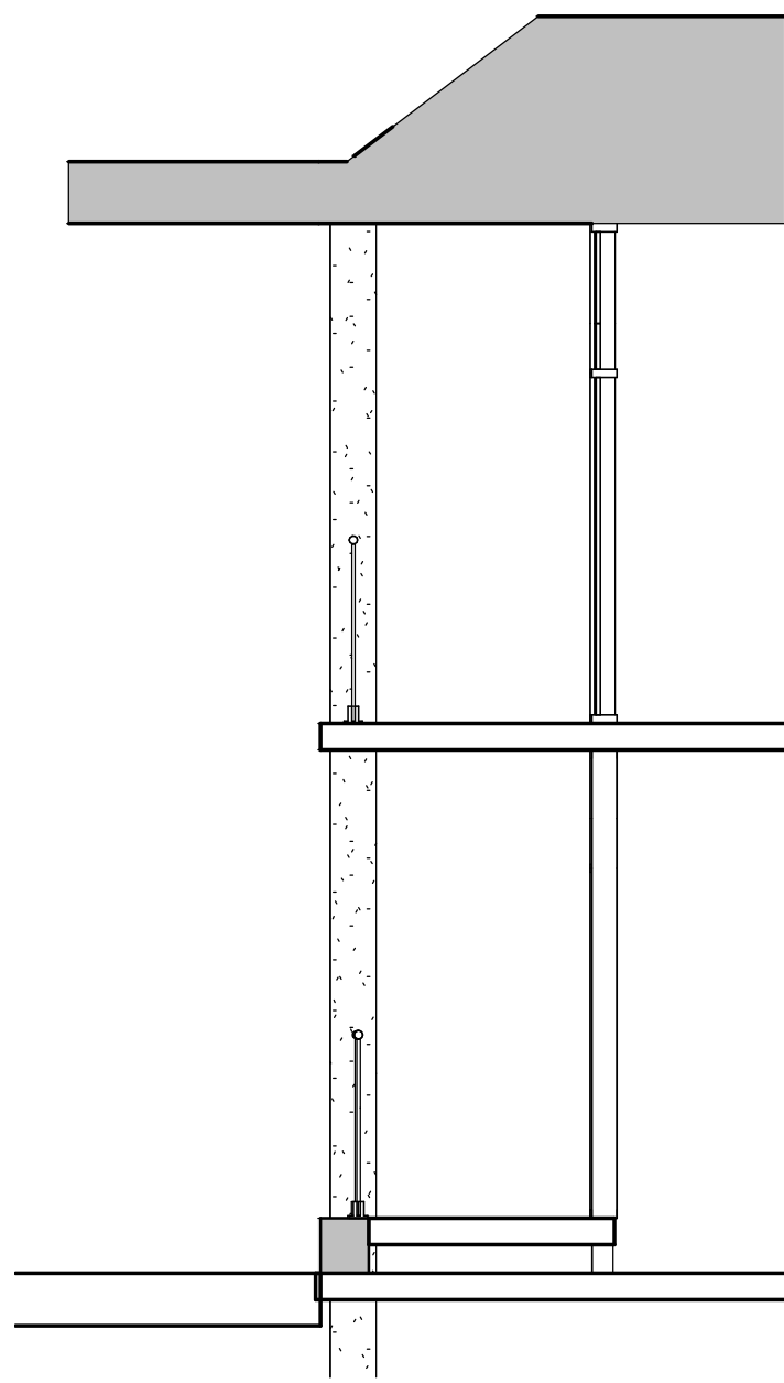
6 Proposed Internal balconies - Detail 1 : 50
