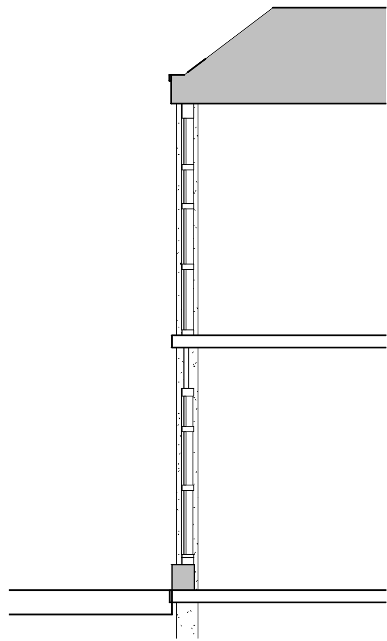
5 Existing South Windows - Detail 1 : 50
