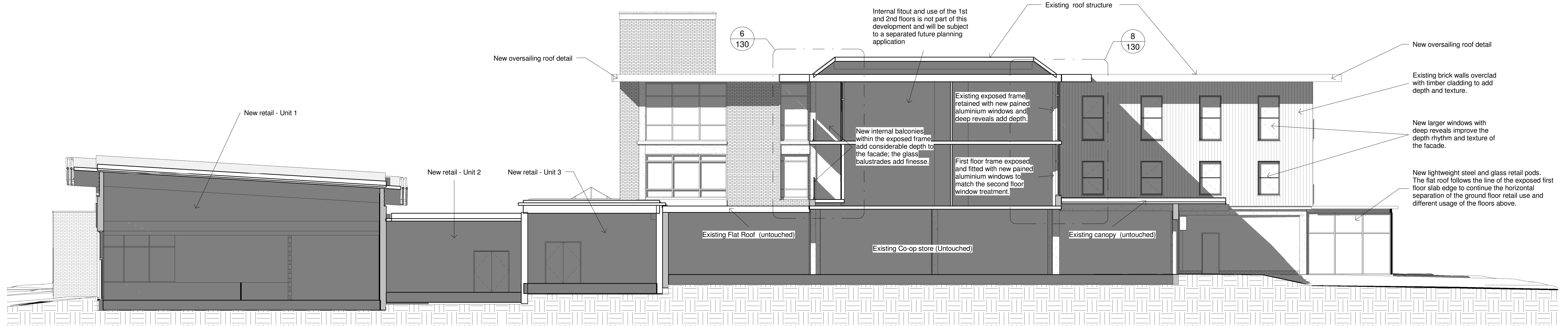
2 Section A - A As Proposed 1 : 100
