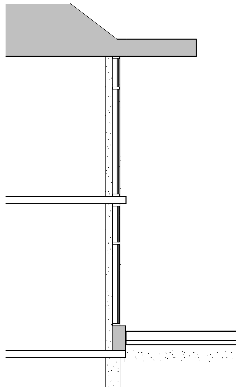
8 Proposed North Window - Detail 1 : 50
