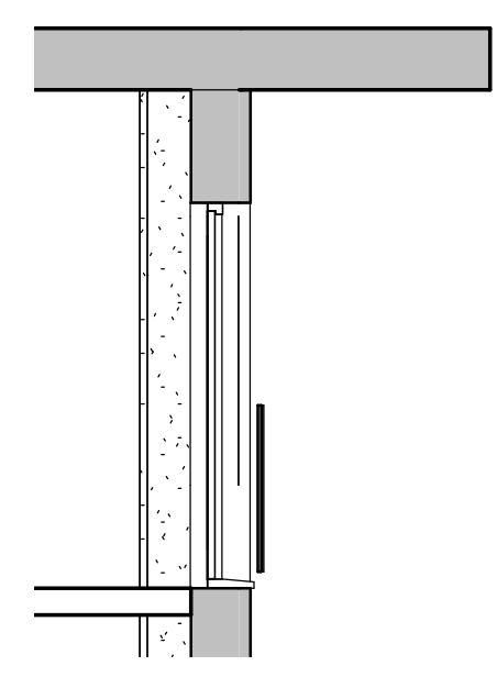
11 Proposed Juliette Balcony - Detail 1 : 50
