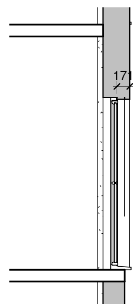
10 Proposed Window - Detail 1 : 50
