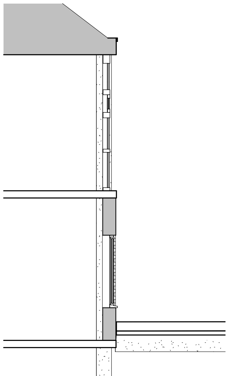
7 Existing North Window - Detail 1 : 50
