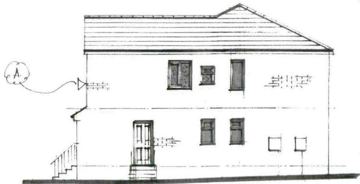
Proposed Side Elevation On 2
