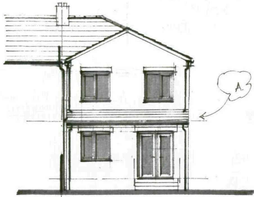
Proposed Rear Elevation On 1
