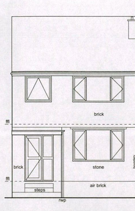
EXISTING ELEVATION A - front (1:100)
