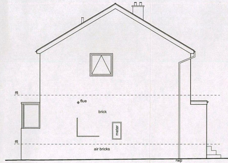
EXISTING ELEVATION C - side (1:100)
