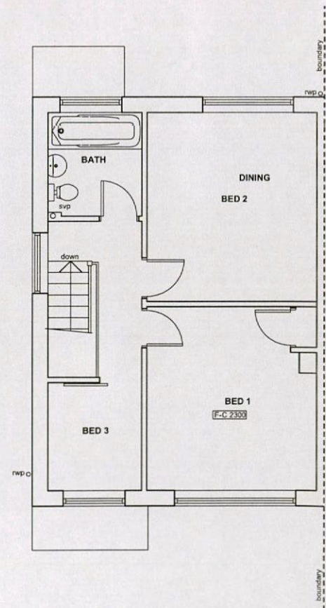
EXISTING FIRST FLOOR PLAN (1:100)
