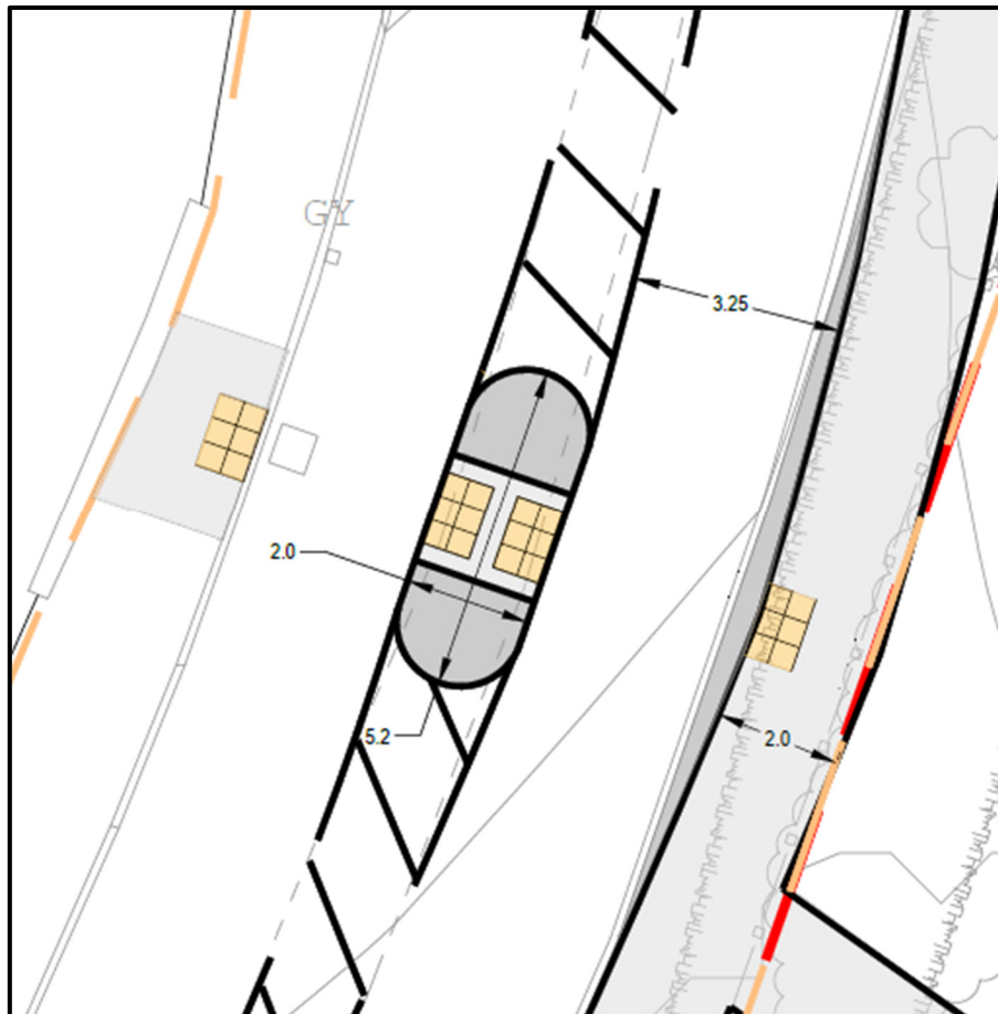
Image 4.3 Proposed Crossing Facility
