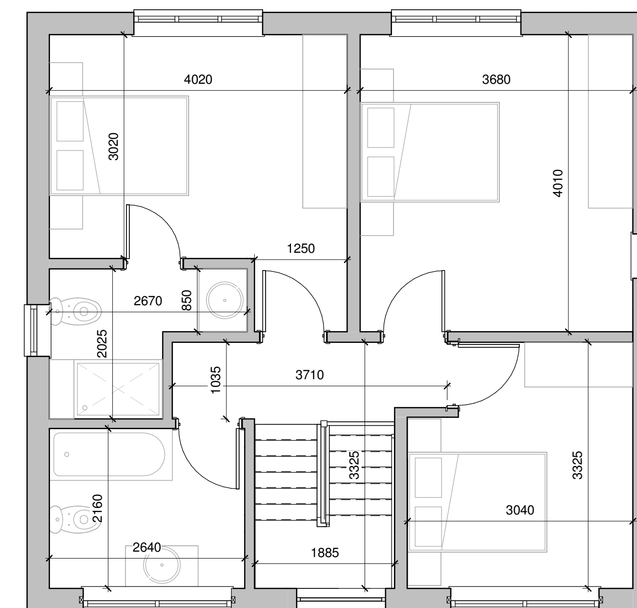
First Floor Level Dimensioned
