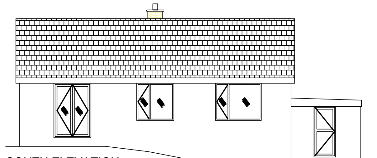
SOUTH ELEVATION
