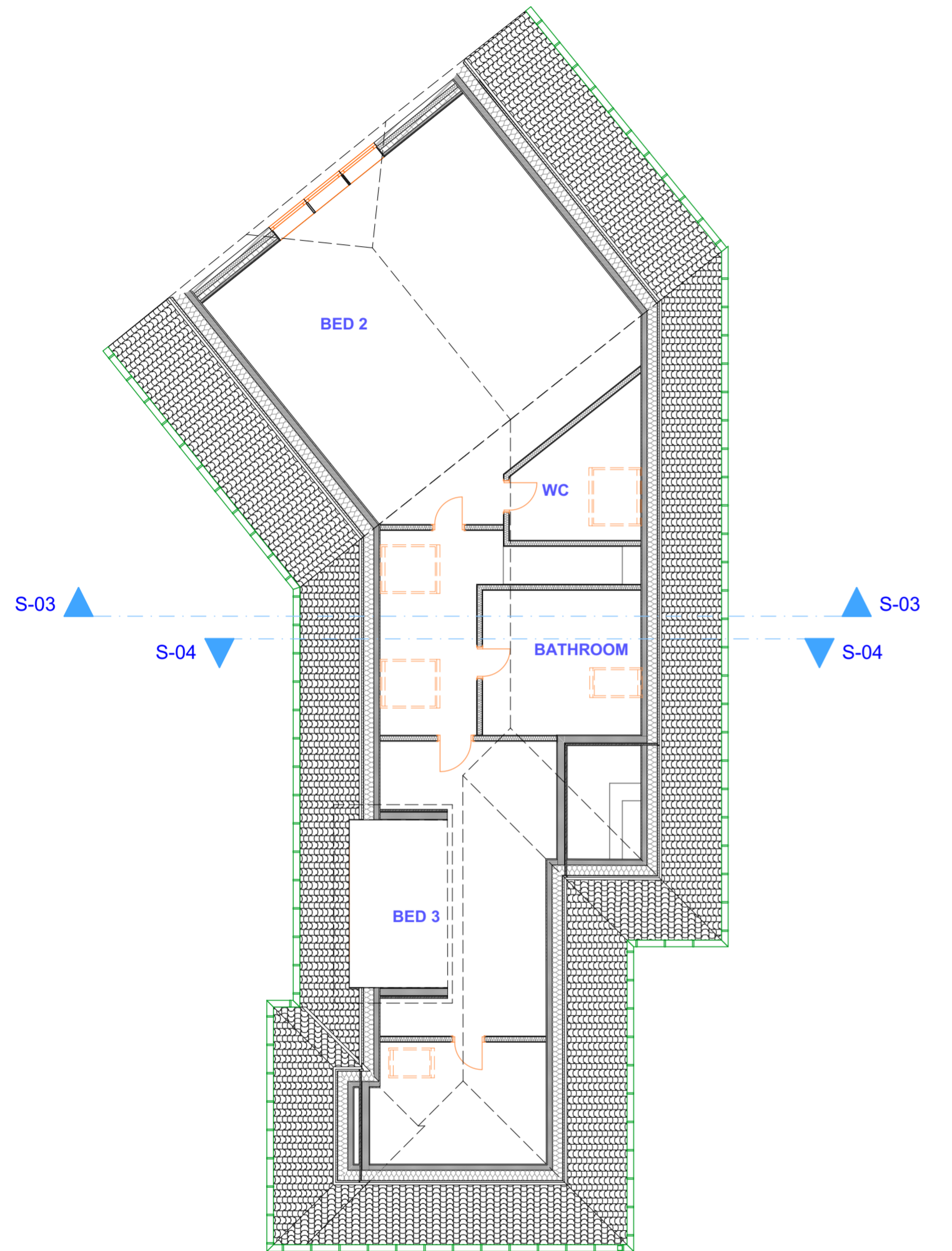
3 1. Loft rooms (1) 1:100
