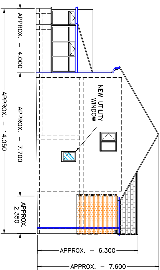
PROPOSED NORTH SIDE ELEVATION
