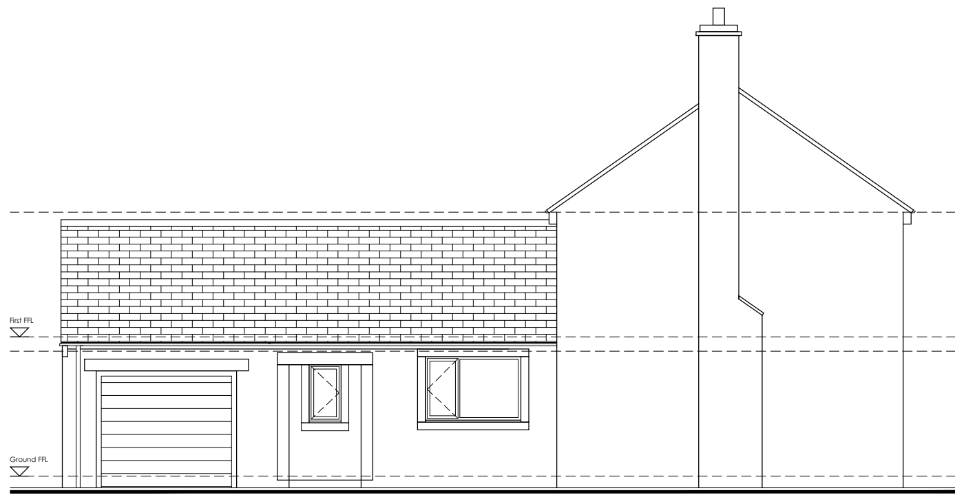
EXISTING FRONT (SSW) ELEVATION 1:100
