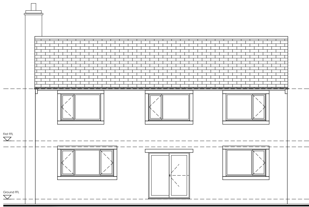
EXISTING SIDE (EES) ELEVATION 1:100
