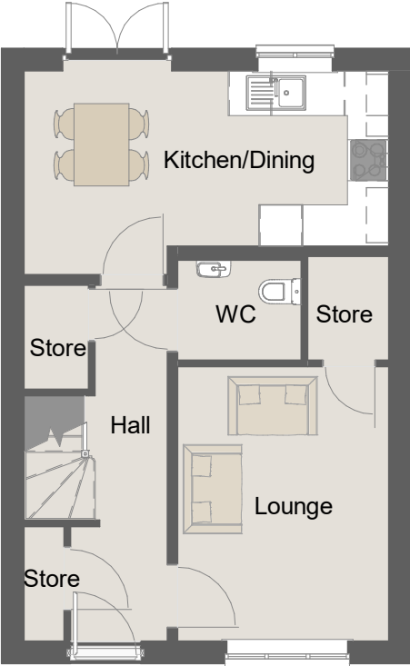
Ground Floor. 1 : 100
