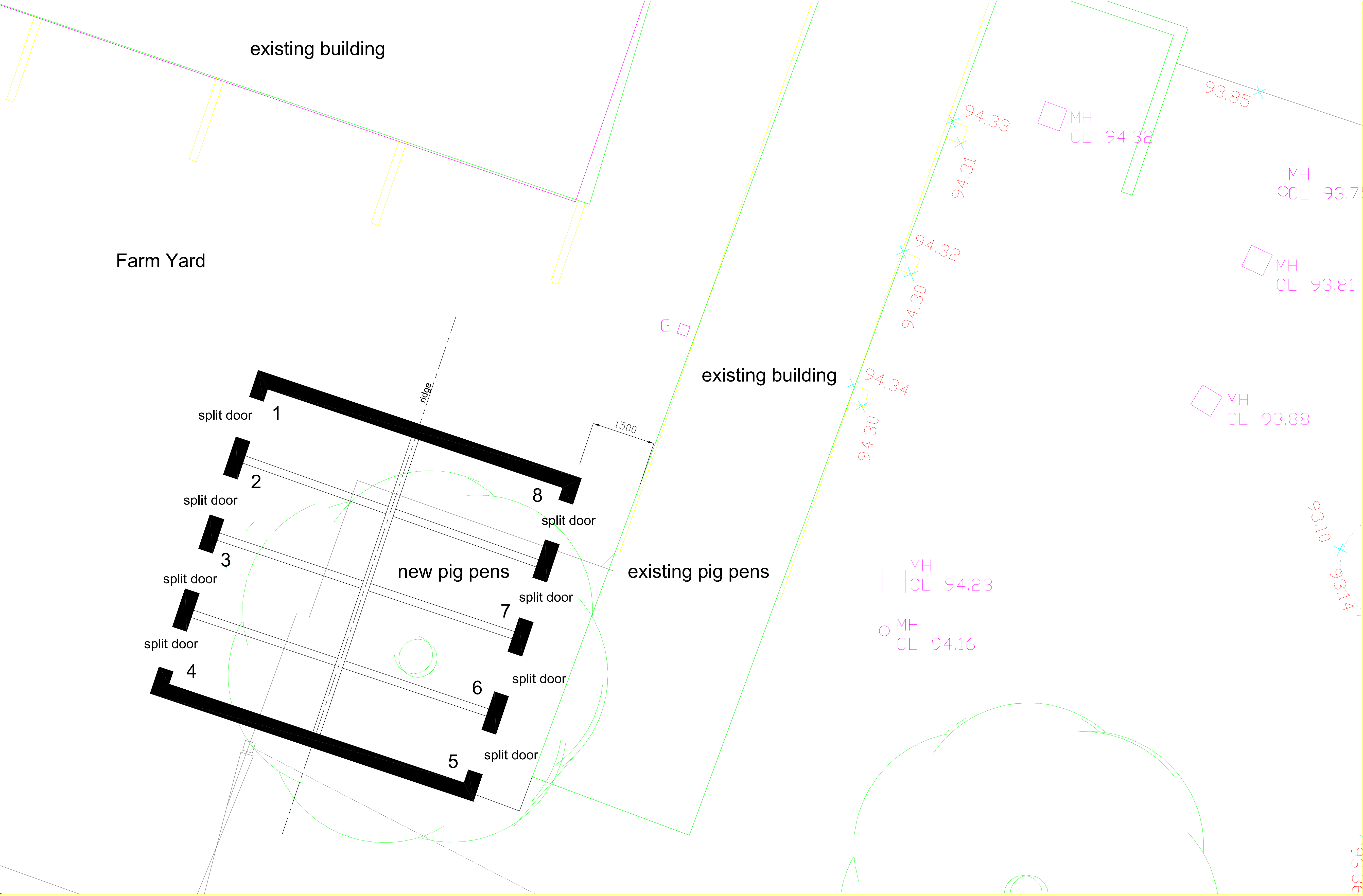
Proposed Plan to Building A scale 1:50
